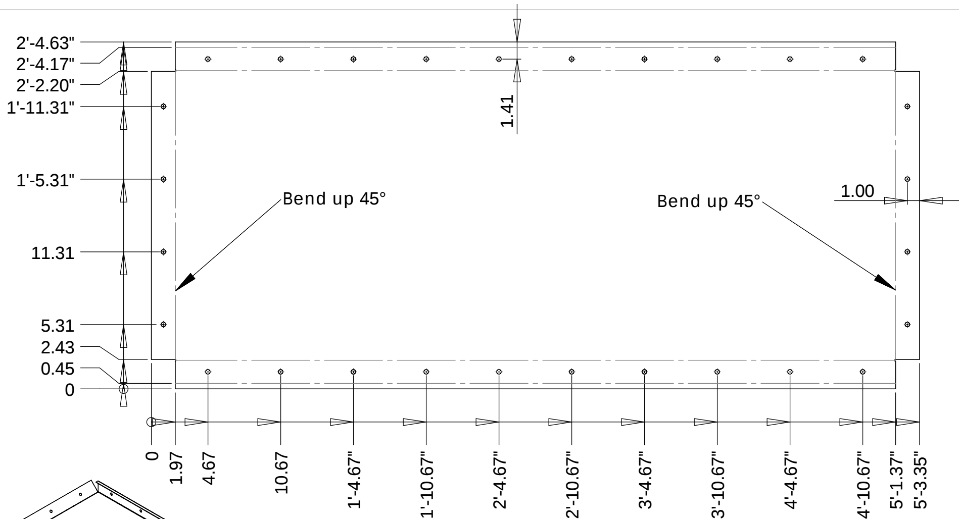
Flat Pattern
